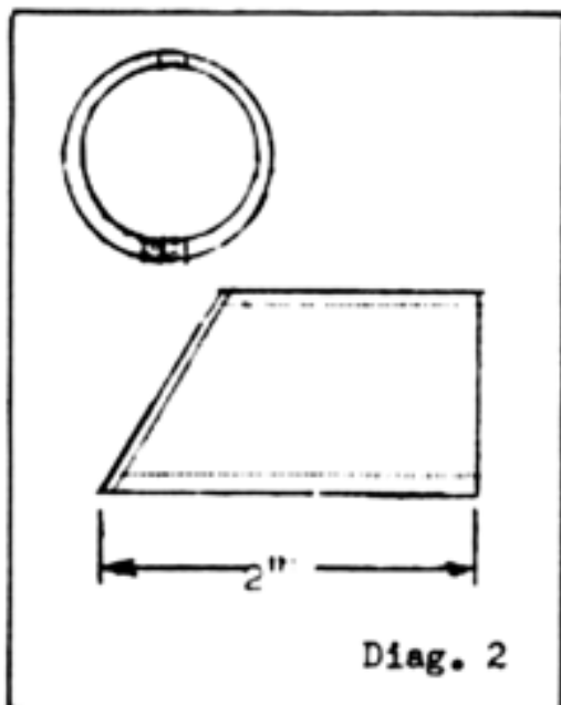
Diagram 2- Drill 1/2" hole in 1/2" brass rod 2" overall length. Drill 1/8" hole at 15 degree angle to furthest end. Cut away excess stock to allow half of hole to show as recess on both ends. Similar type tube made with .025 wall. Any nut with 1/4 x 20 threads to act as lock.
