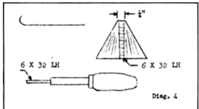
Diagram 4— (Tone Hole Undercutting Tool) Circular file or deburring tool. 1/2" diameter at large end. Soften or anneal. Remove back stud. Drill hole with No. 36 drill. Thread 6 x 32. Face off small end to 3/16". Thread must be left hand. Screw driver holder threaded on end 6 x 32 left hand. Small hook bent approximate right angle hook end ~46. Wire to be 1/8" drill rod. Hook circular file on wire, large end down. Insert in clarinet to desired tone hole. Screw in from face of tone hole and revolve handle left hand. Upon completion of cutting, reverse handle and remove same.
