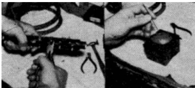
Removing broken springs with special pivot point pliers. Punching out broken piece of spring in lead block.
